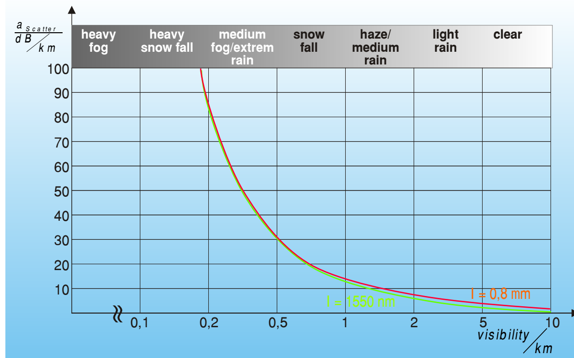
Picture 17: Weather dependent attenuation and the scatter attenuation versus visibility
